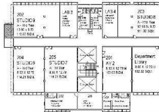
FIRST FLOOR PLAN (B.ARCH. BUILDING)
